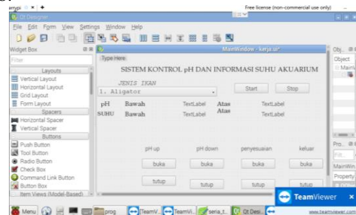
Gambar 18 Tampilan PyQt
