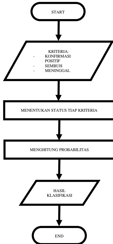
Gambar 2. Flowchart sistem
