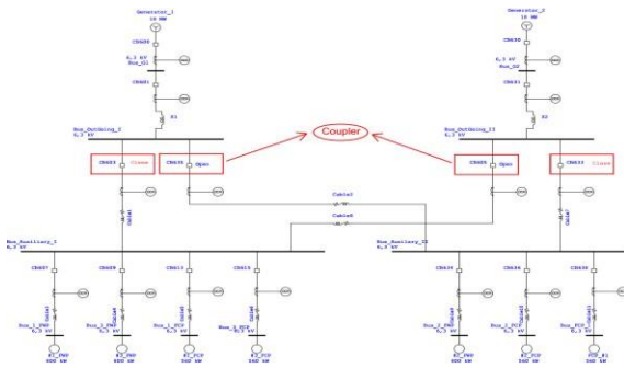
Gambar 2 Pemodelan Single Line Diagram Jaringan Distribusi PS 6.3 kV
